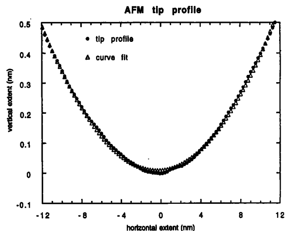
FIG. 2. A tip image acquired from scanning the \text{SrTiO}_3(305) surface in air, taken before the tip was placed in vacuum and the data in Fig. 1 acquired. The actual tip profile is plotted with solid circles, and a parabolic fit is plotted with open triangles for comparison. The tip profile is essentially parabolic, with an effective tip radius of \sim 140 nm.
